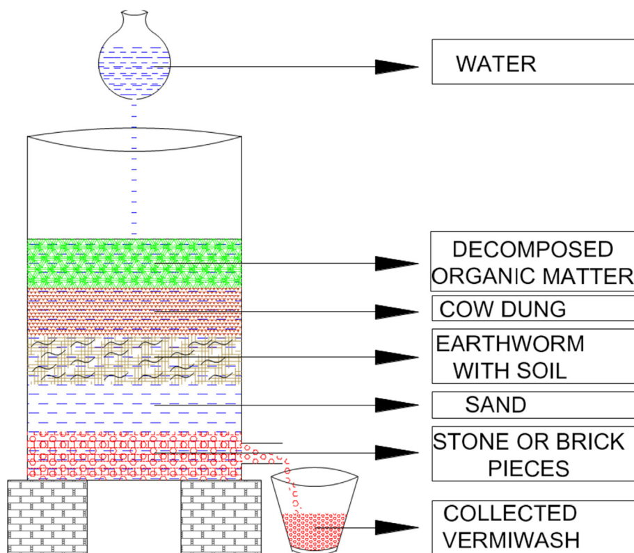
Figure 1. Preparation of vermiwash. It showed a basic means of vermiwash preparation. The bottom layer contains stone or brick pieces in coarse grain. The next layer contains sand, which helps to drain water through it to maintain moderate moisture. In the third layer earthworms inoculated with organic soil, in the fourth layer cow dung, or any organic waste which used as a main raw material. On the top layer the decomposed organic matter such as leaf litter, straw, etc an additional raw material that mainly prevents direct exposure from sunlight. The periodic sprinkling of water should be done to prevent desiccation and facilitate the comminution of organic matter. Finally, pure vermiwash harvested for application.
